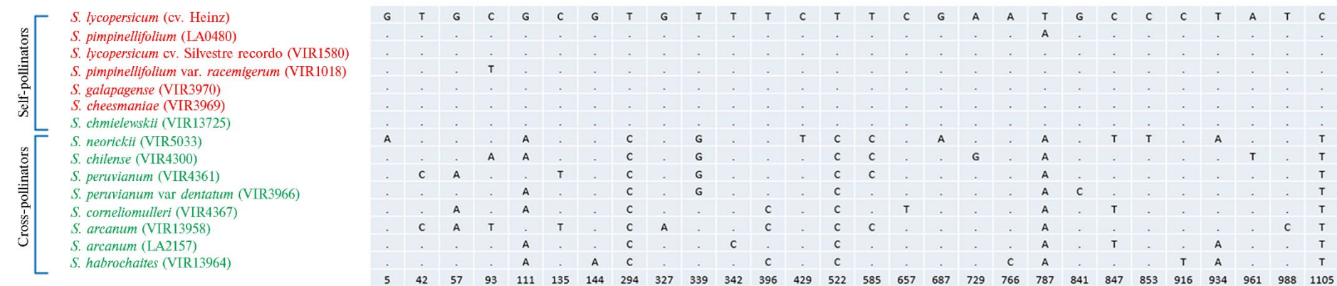
Fig. 2. Distribution of SNPs in the coding region of GME1 homologues genes in the studied cross- and self-pollinated wild-growing species and varieties of tomato ( Solanum L.). Numerical values indicate the location of single nucleotide substitutions. See the description of species and varieties in the Materials and methods and in Table 1.
